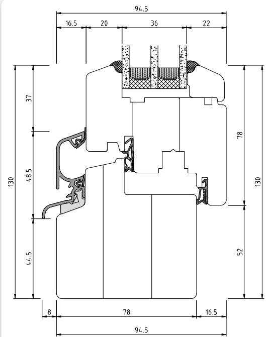
WOODEN WINDOW IV 78 PROFILE SECTION
