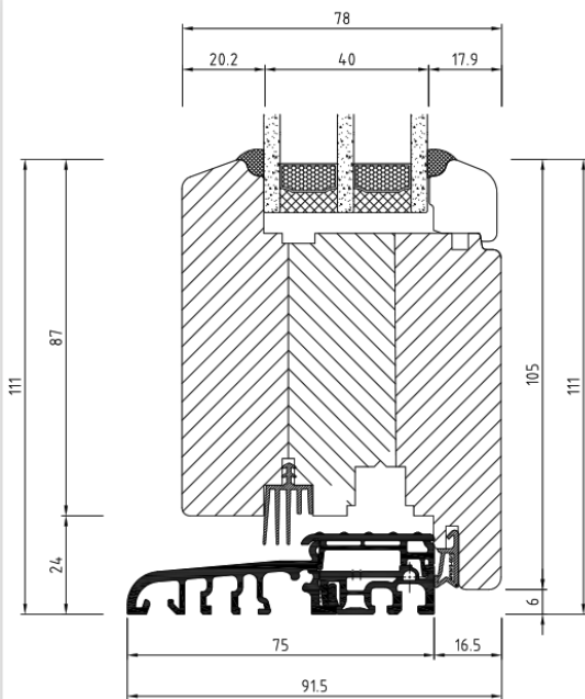
IV 78 FRENCH DOOR WITH FLAT THRESHOLD
